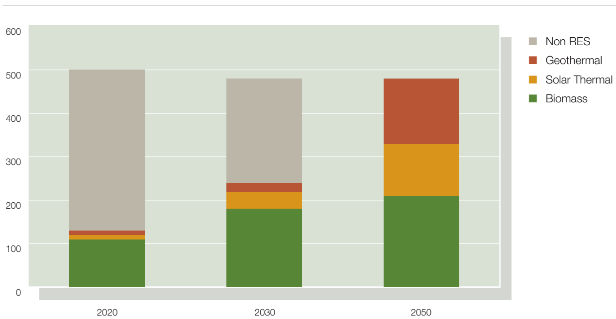
Figure 10 Contribution of Renewable Heating and Cooling Technologies to Heat Consumption (Mtoe)
